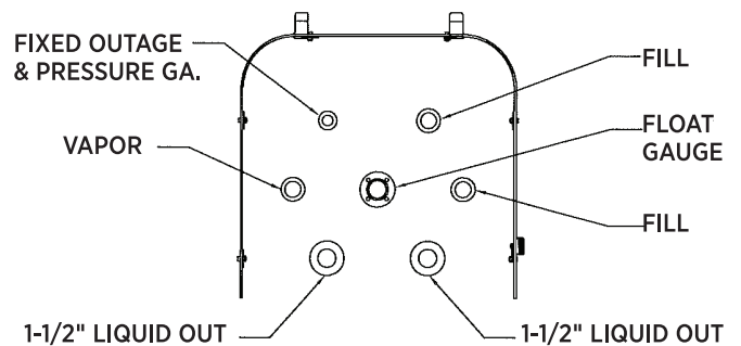
FITTING LAYOUT UNDER FITTING COVER
