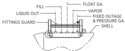
STANDARD FITTINGS ARRANGEMENT 1,000 wg \ 1,465 wg \ 2,000 wg TOP-FIT (Relief Valve (s) not shown)
